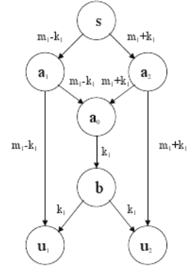
Fig. 2. Cai and Yeung's private network coding
