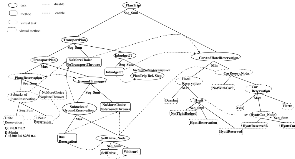
Figure 4: TÆMS Task Structure for PlanTrap Example
