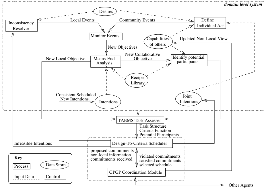
Figure 6: BDI Agent Architecture with coordination module
